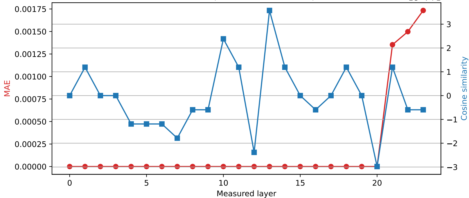
SmolLM2-1.7B-Instruct | Quantized layer 20 | float32 → int16
