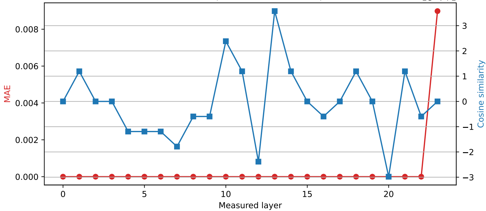
SmolLM2-1.7B-Instruct | Quantized layer 22 | float32 → int16
