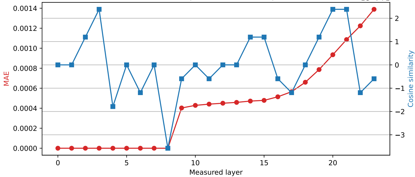
SmolLM2-1.7B-Instruct | Quantized layer 8 | float32 \rightarrow int16
