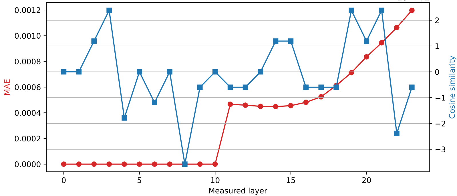
SmolLM2-1.7B-Instruct | Quantized layer 10 | float32 \rightarrow int16
