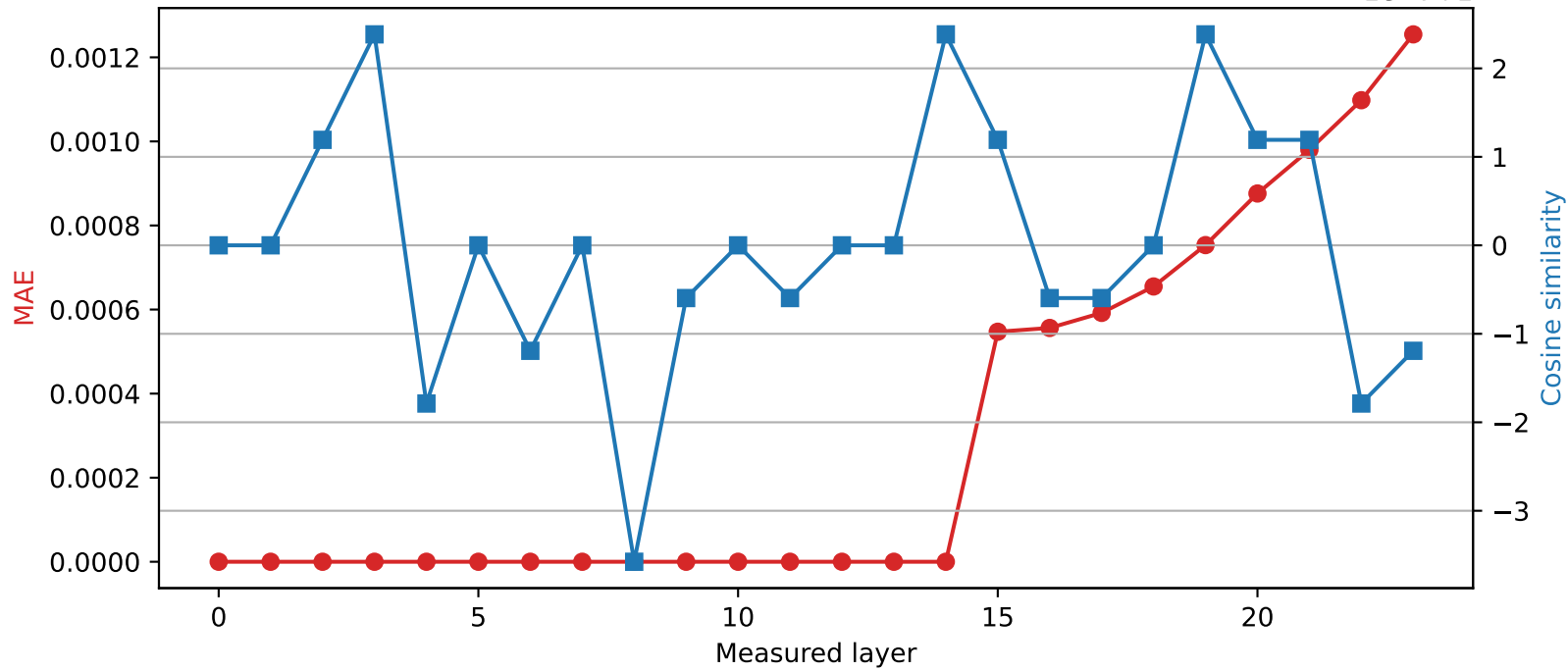
SmolLM2-1.7B-Instruct | Quantized layer 14 | float32 → int16
