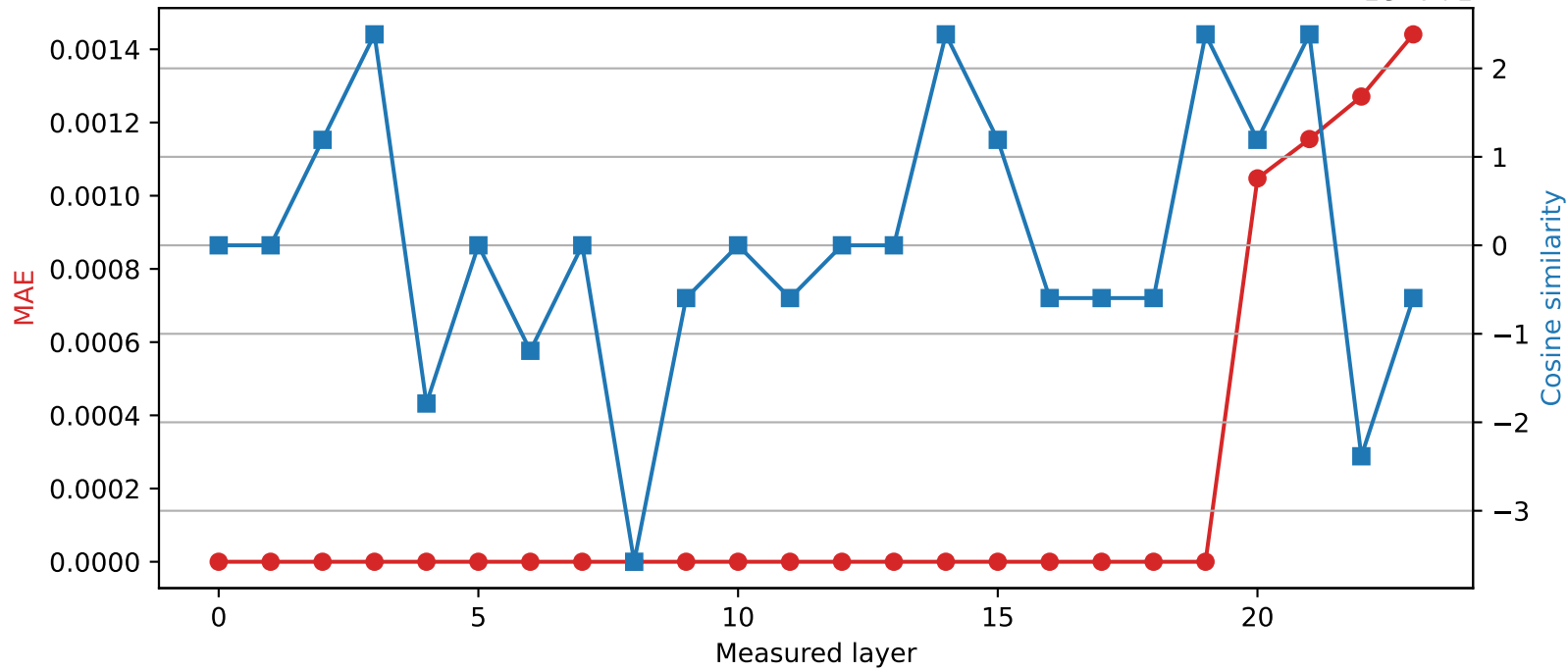
SmolLM2-1.7B-Instruct | Quantized layer 19 | float32 \rightarrow int16
