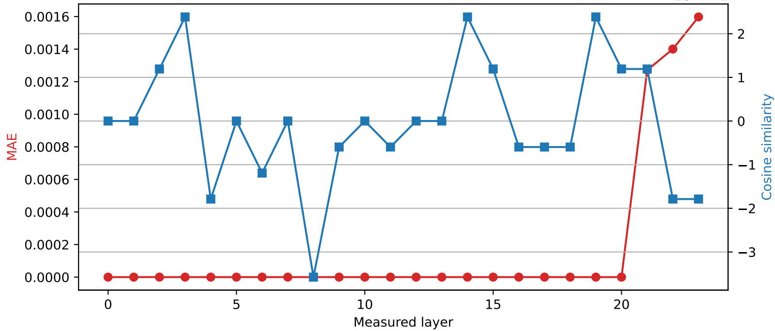
SmolLM2-1.7B-Instruct | Quantized layer 20 | float32 \rightarrow int16
