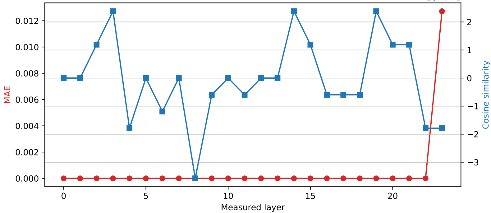
SmolLM2-1.7B-Instruct | Quantized layer 22 | float32 \rightarrow int16
