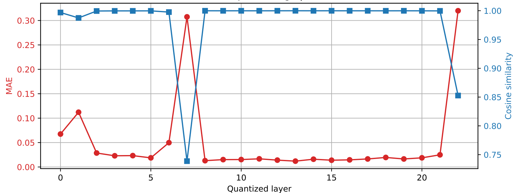
SmolLM2-1.7B-Instruct | Prompt 0 Final RMSNorm output damage | float32 → int8
