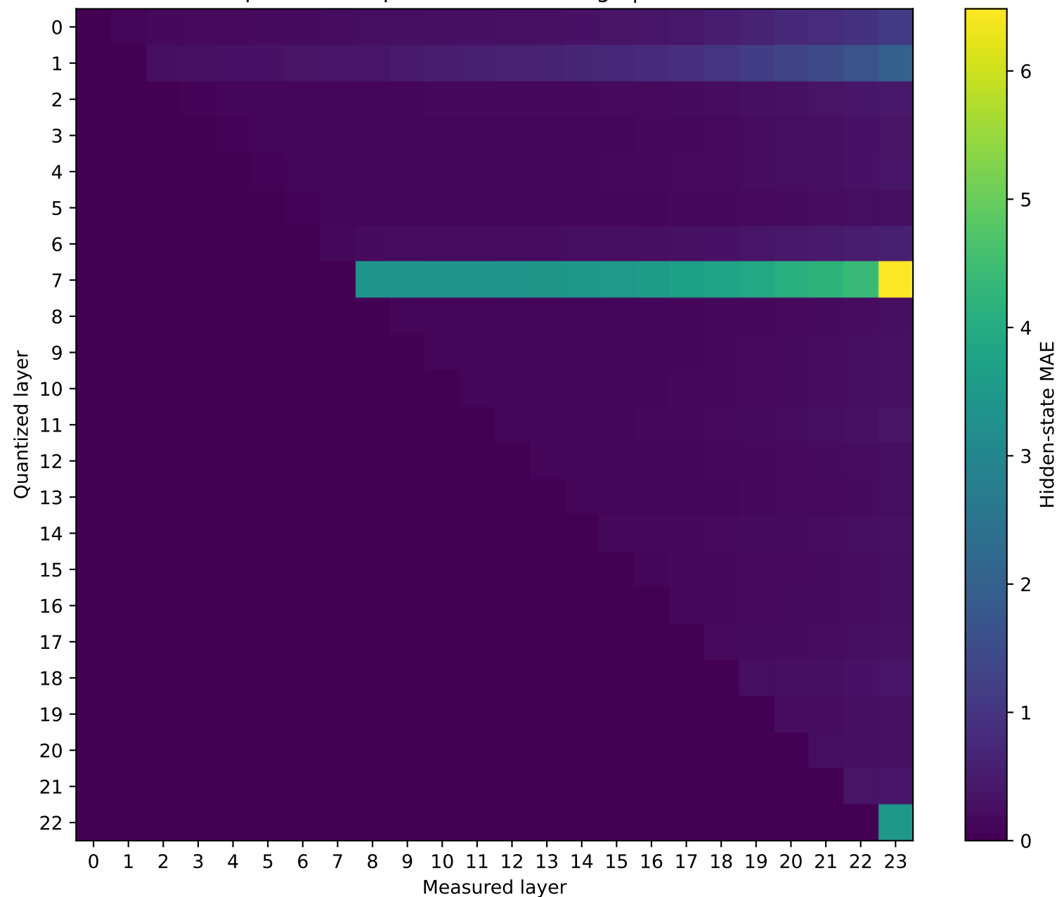
SmolLM2-1.7B-Instruct Prompt 0: MAE representation damage | float32 → int8
