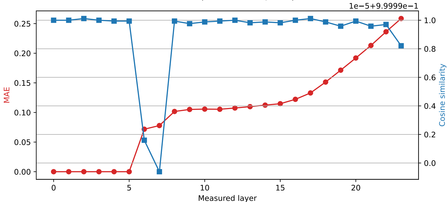
SmolLM2-1.7B-Instruct | Quantized layer 5 | float32 \rightarrow int8
