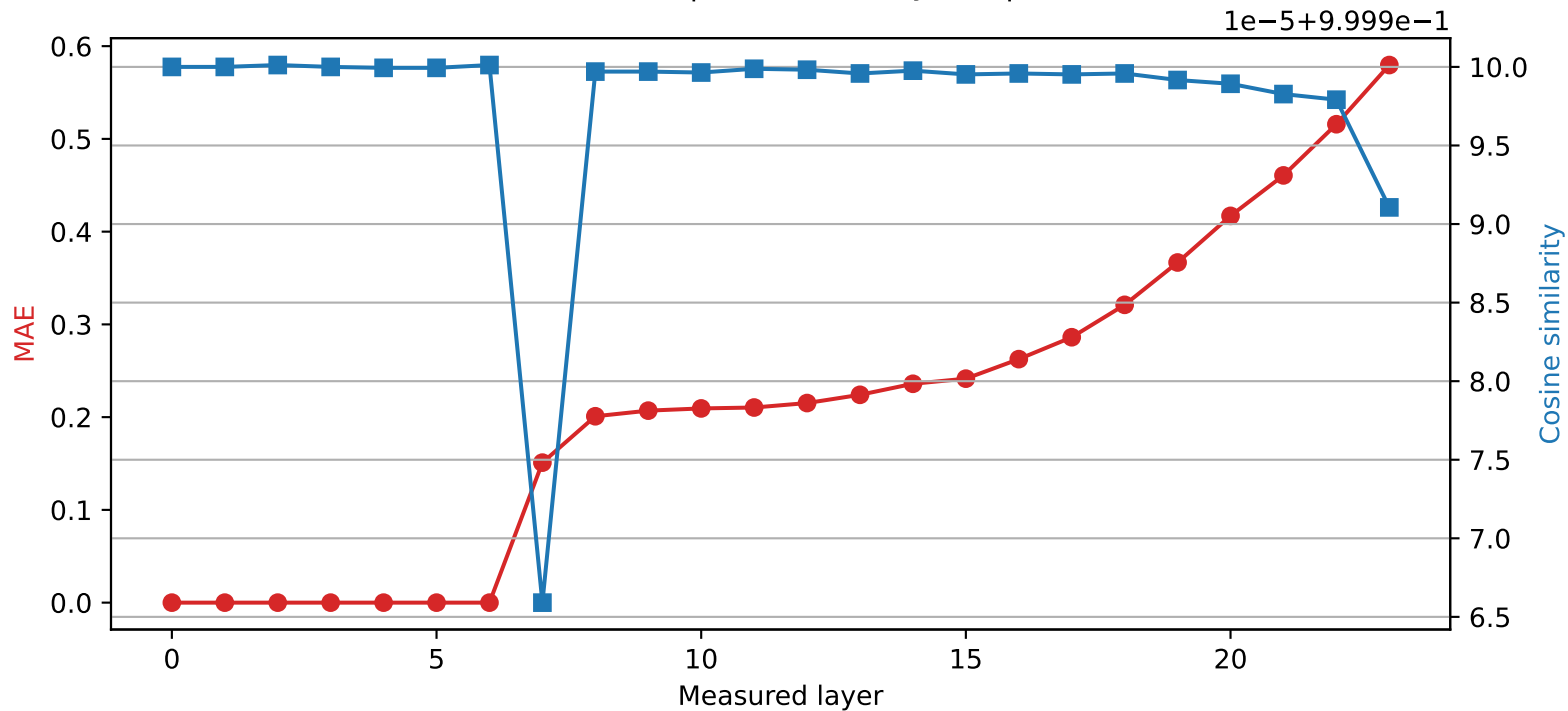
SmolLM2-1.7B-Instruct | Quantized layer 6 | float32 \rightarrow int8
