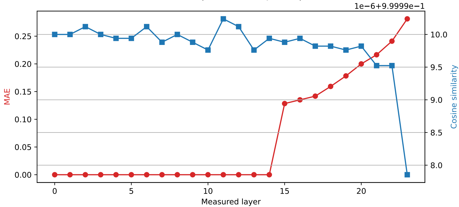
SmolLM2-1.7B-Instruct | Quantized layer 14 | float32 → int8
