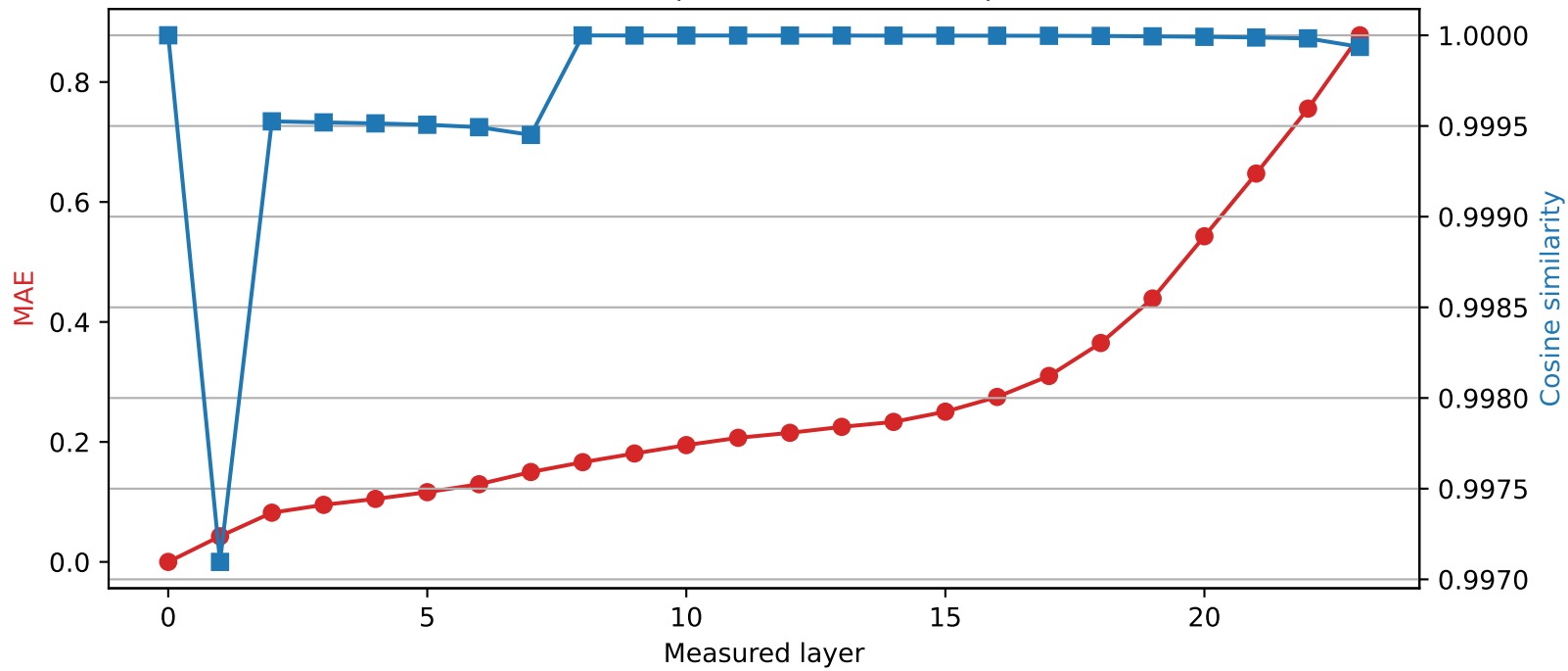
SmolLM2-1.7B-Instruct | Quantized layer 0 | float32 → int8
