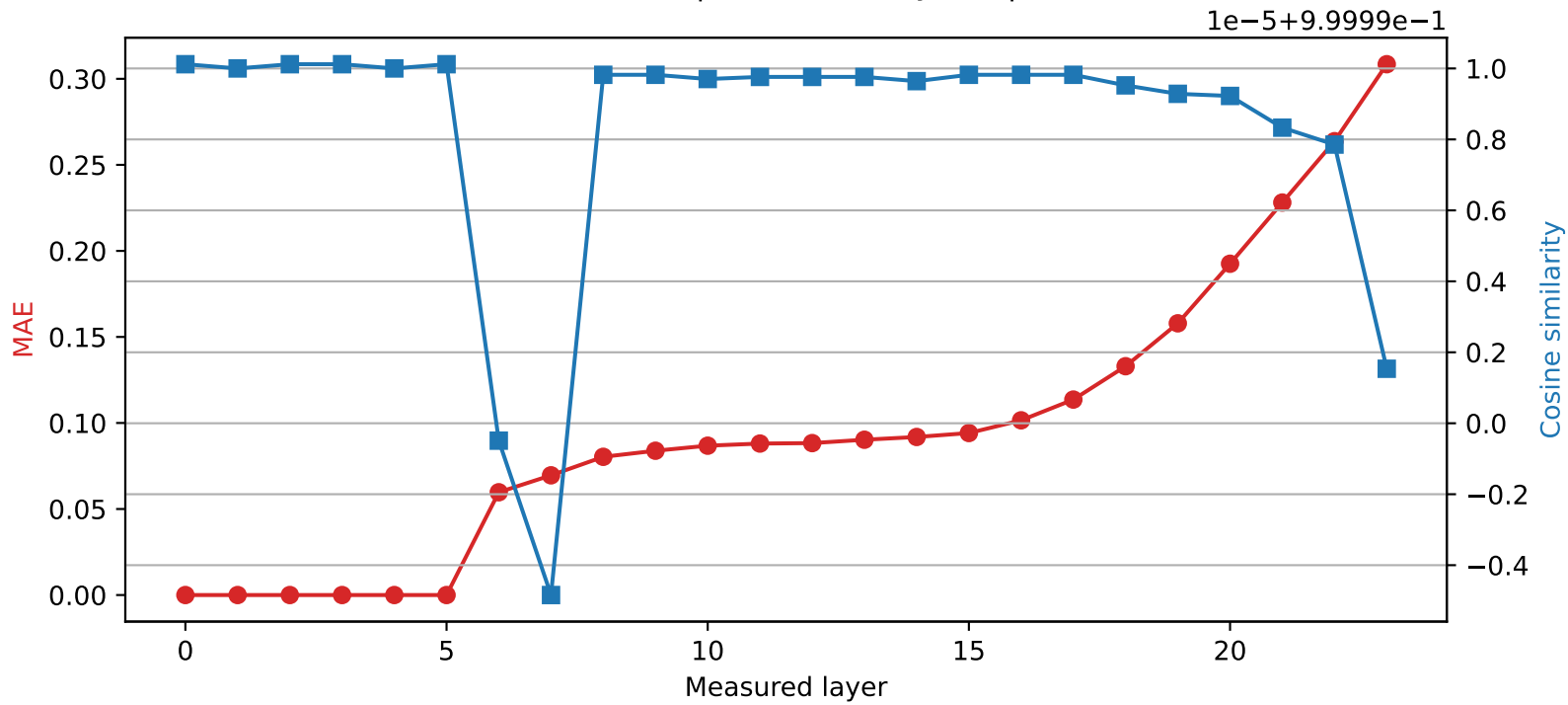
SmolLM2-1.7B-Instruct | Quantized layer 5 | float32 → int8
