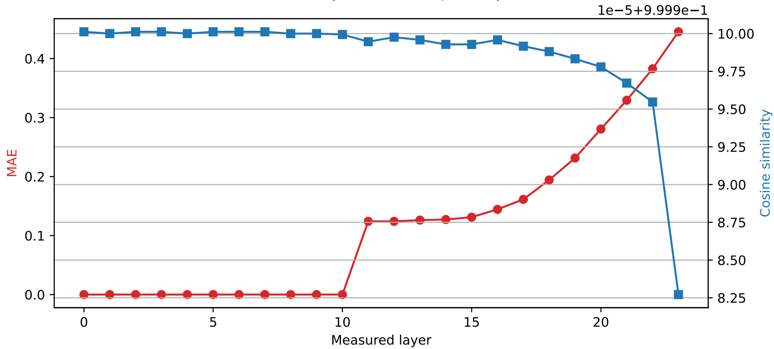
SmolLM2-1.7B-Instruct | Quantized layer 10 | float32 → int8
