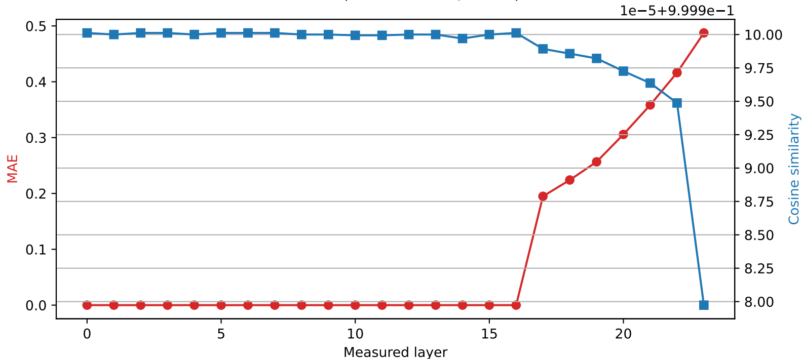
SmolLM2-1.7B-Instruct | Quantized layer 16 | float32 → int8
