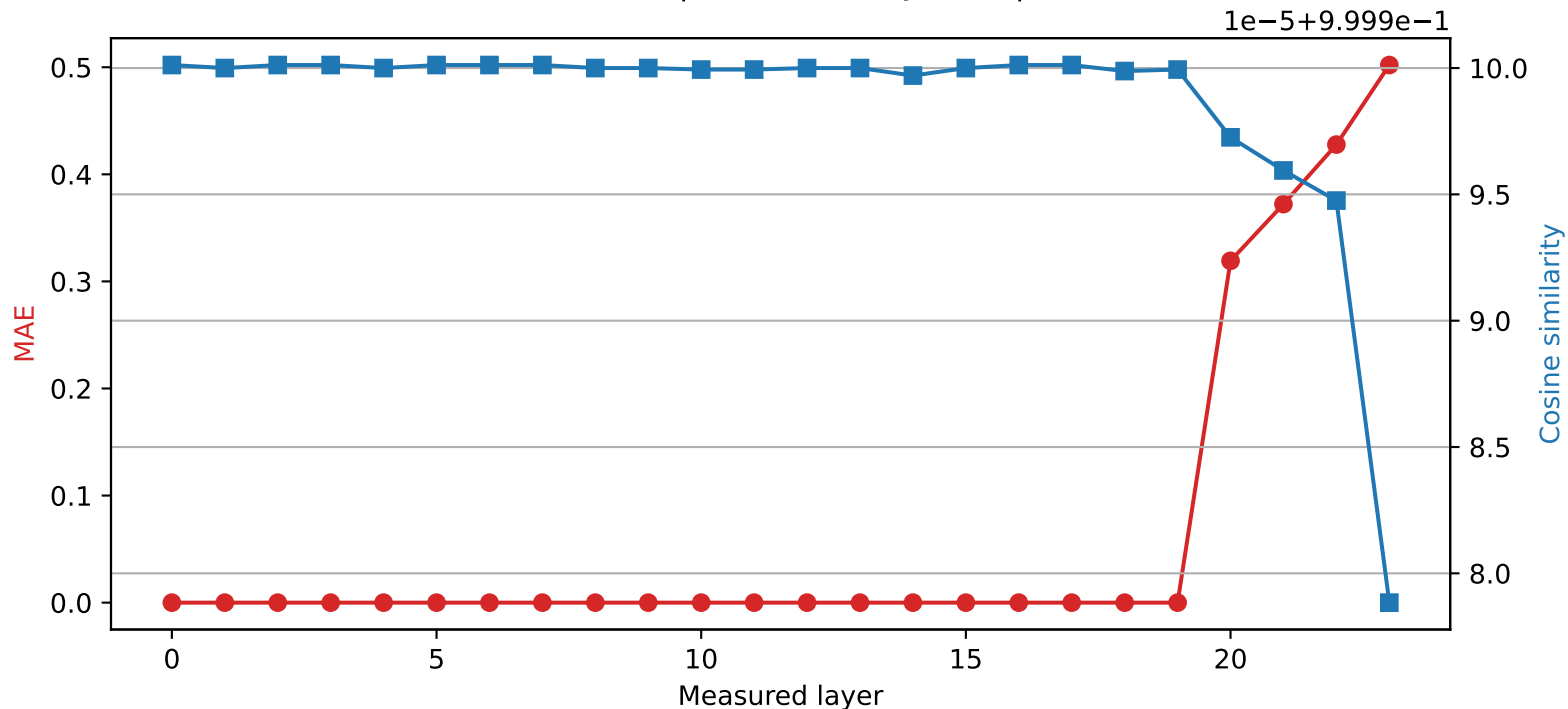
SmolLM2-1.7B-Instruct | Quantized layer 19 | float32 → int8
