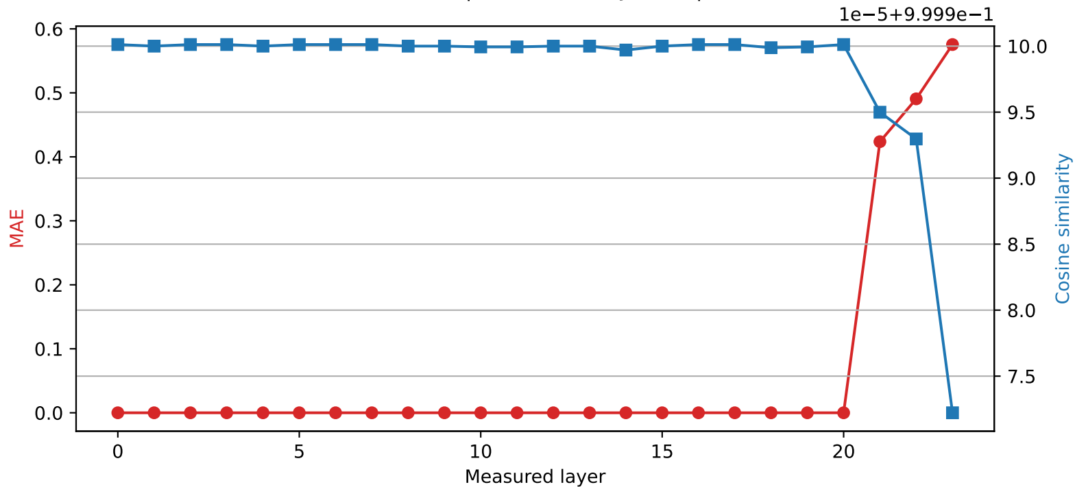
SmolLM2-1.7B-Instruct | Quantized layer 20 | float32 \rightarrow int8
