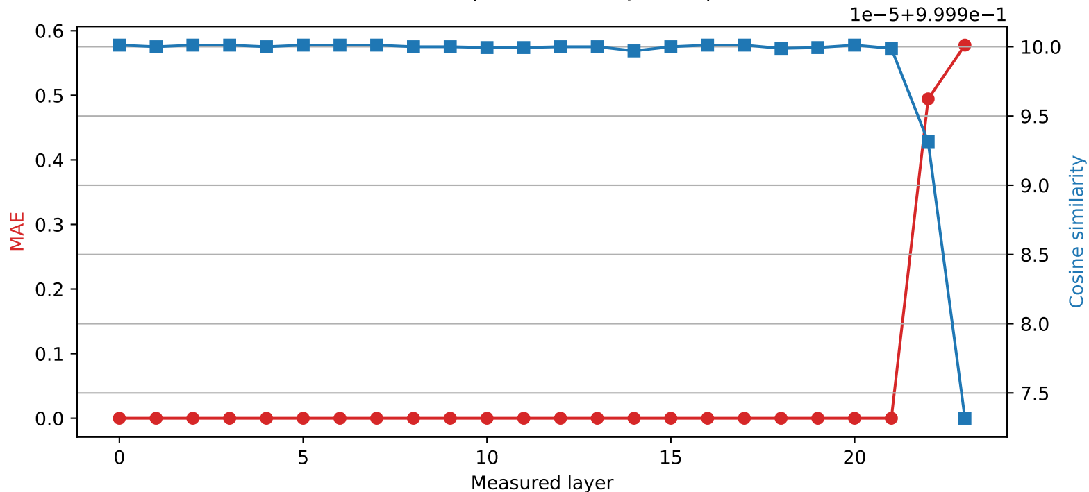
SmolLM2-1.7B-Instruct | Quantized layer 21 | float32 \rightarrow int8
