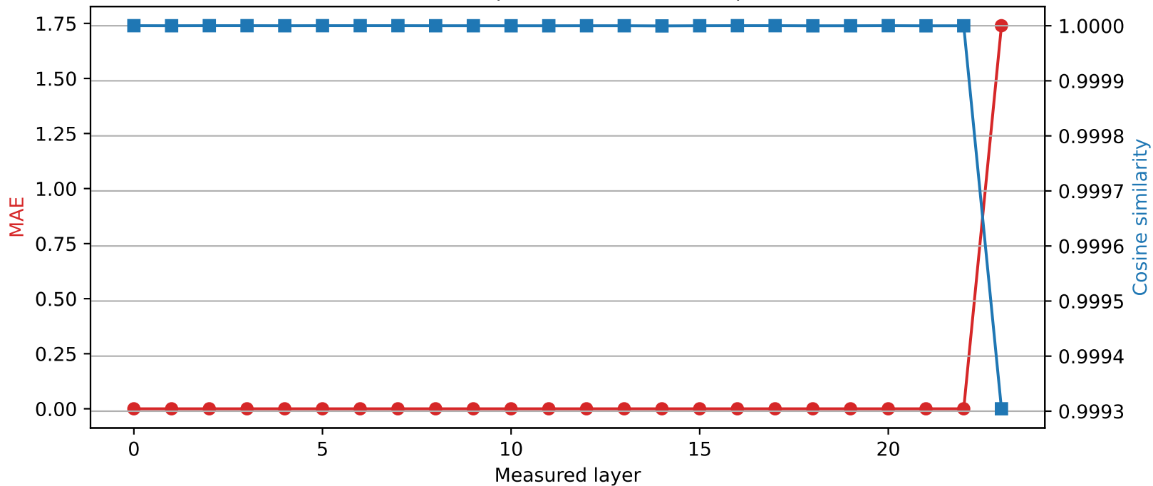
SmolLM2-1.7B-Instruct | Quantized layer 22 | float32 \rightarrow int8
