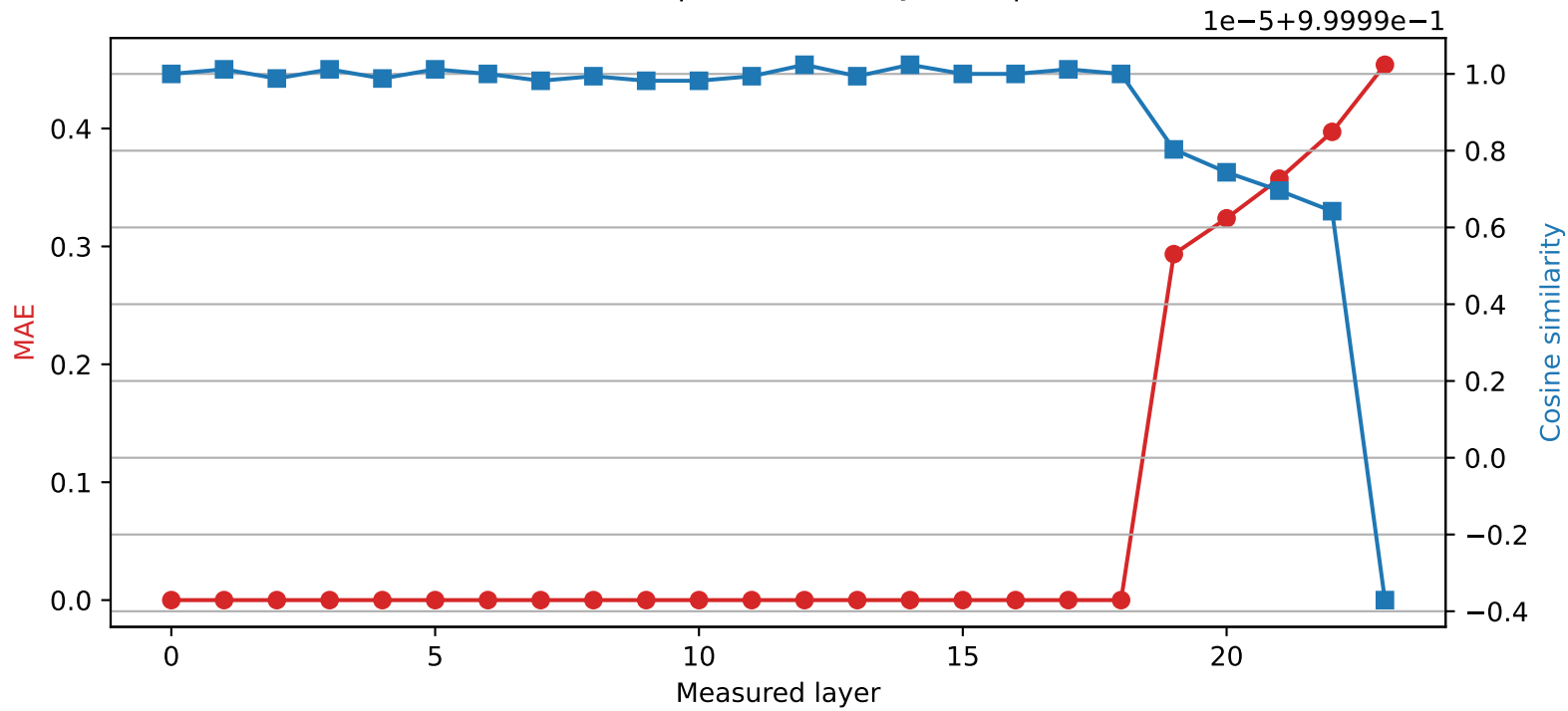
SmolLM2-1.7B-Instruct | Quantized layer 18 | float32 \rightarrow int8
