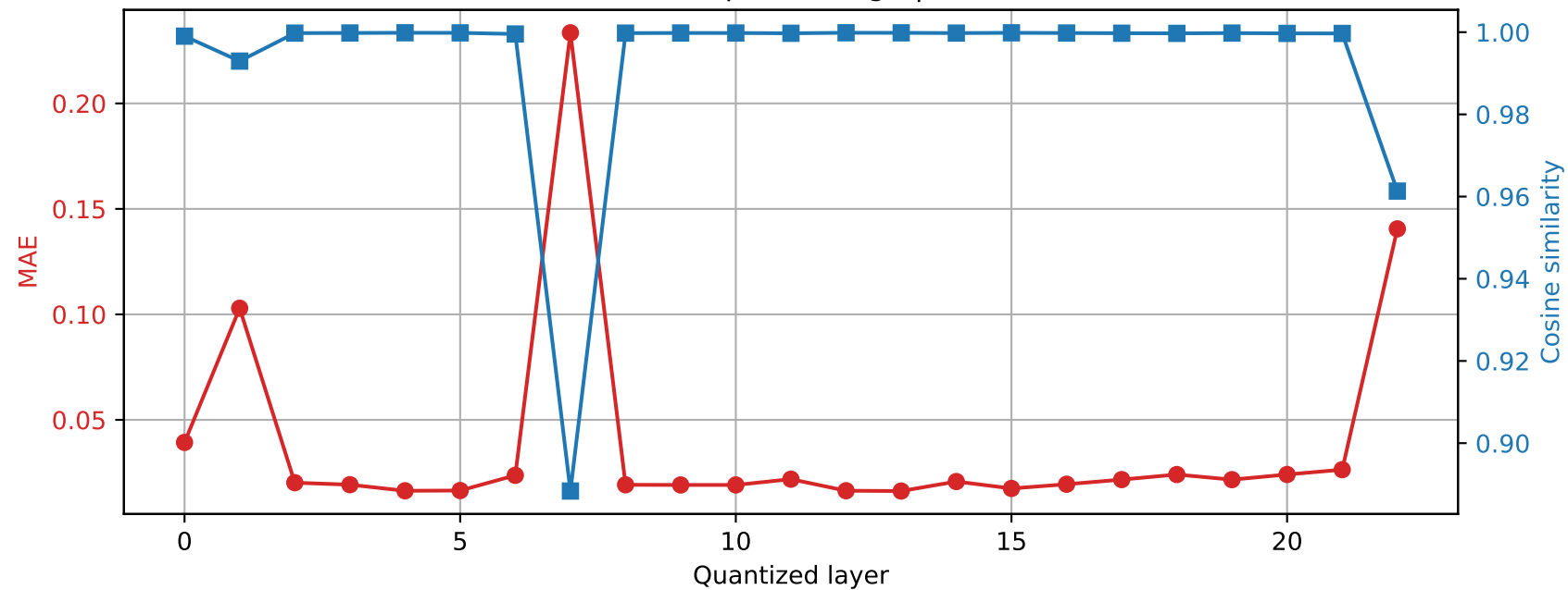
SmolLM2-1.7B-Instruct | Prompt 3 Final RMSNorm output damage | float32 \rightarrow int8
