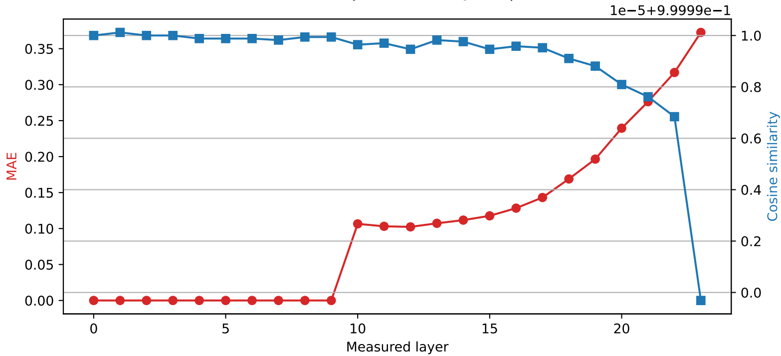
SmolLM2-1.7B-Instruct | Quantized layer 9 | float32 → int8
