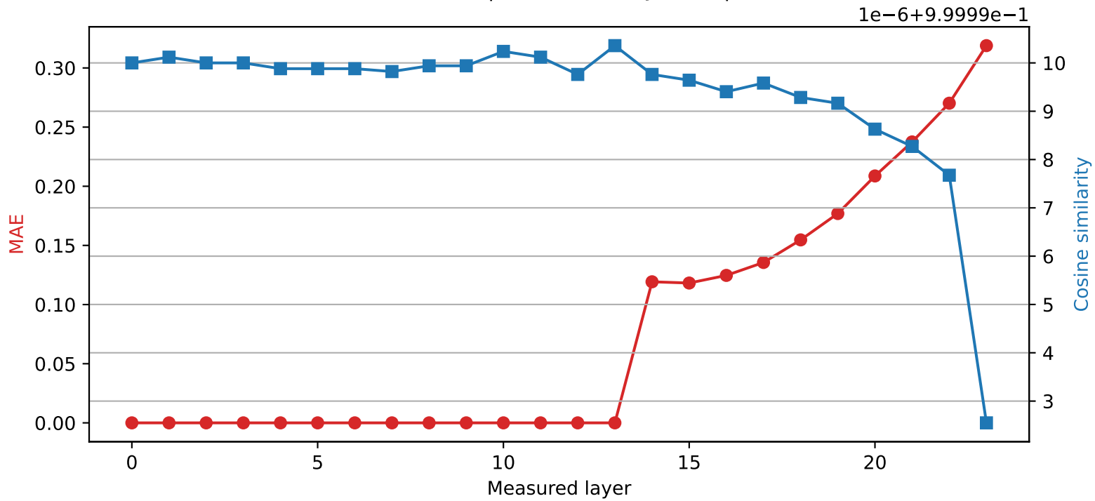
SmolLM2-1.7B-Instruct | Quantized layer 13 | float32 \rightarrow int8
