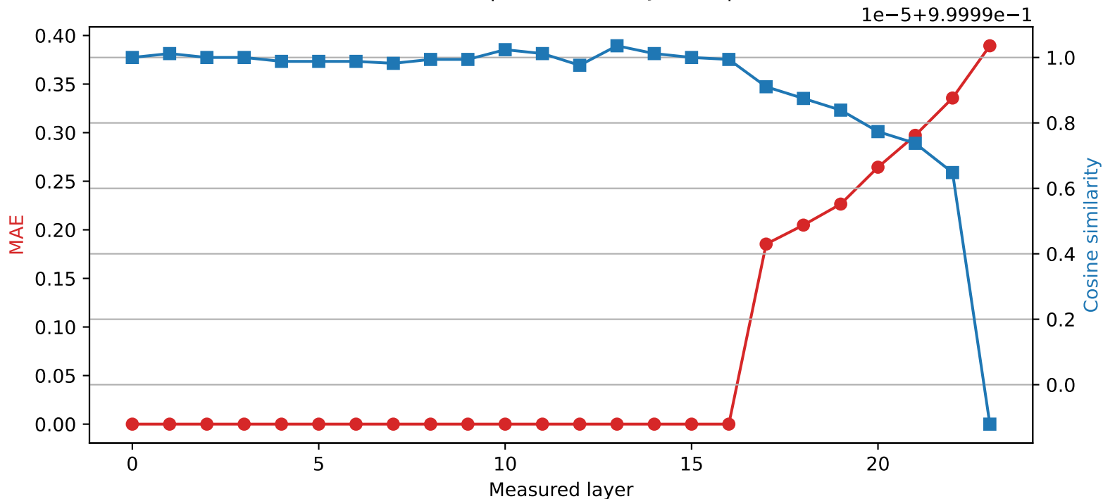
SmolLM2-1.7B-Instruct | Quantized layer 16 | float32 \rightarrow int8
