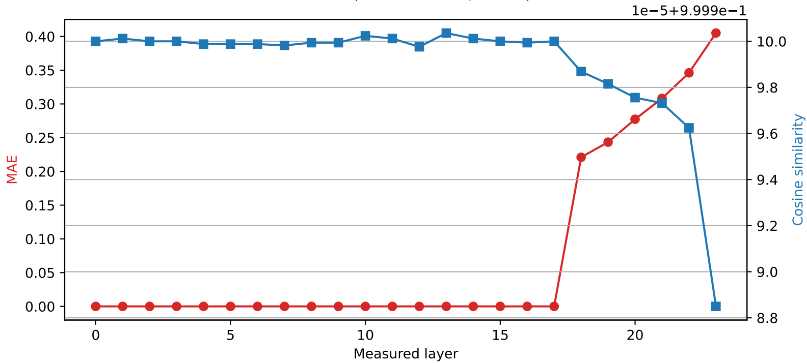
SmolLM2-1.7B-Instruct | Quantized layer 17 | float32 \rightarrow int8
