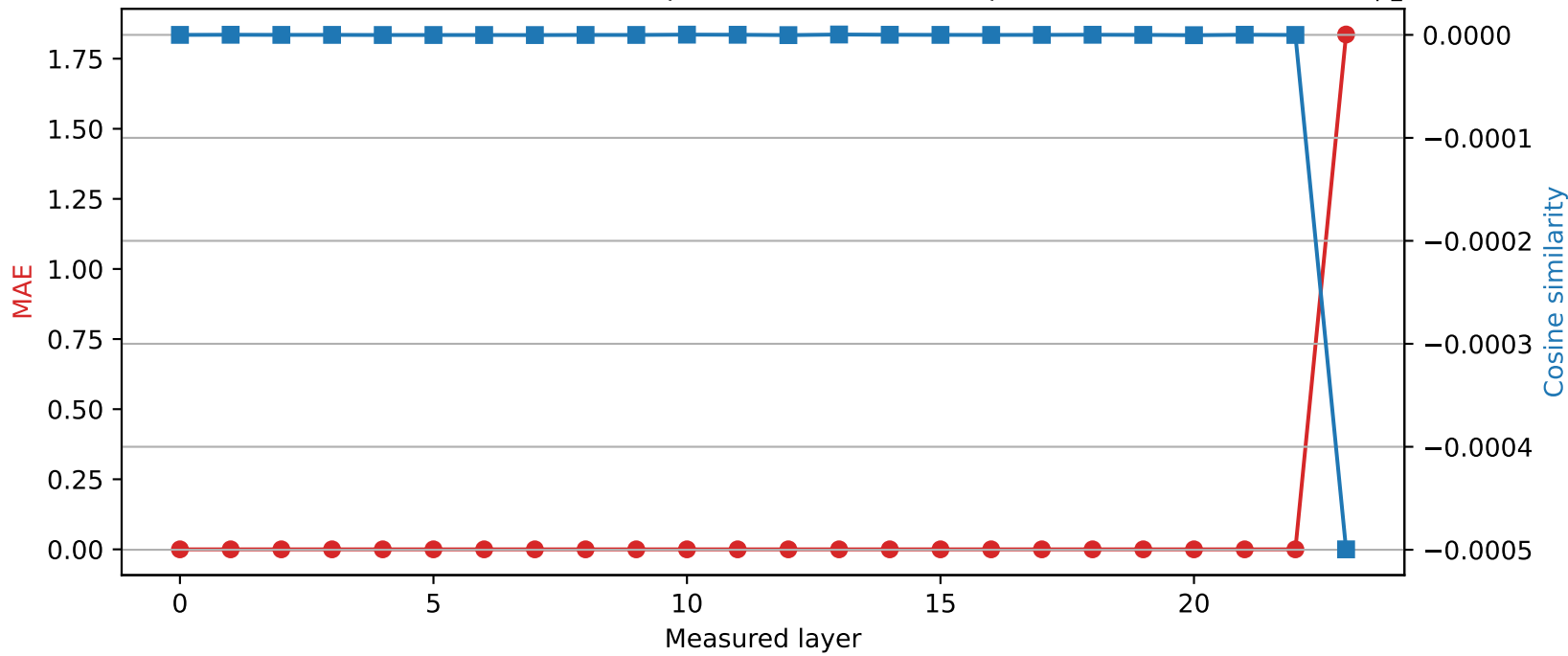
SmolLM2-1.7B-Instruct | Quantized layer 22 | float32 \rightarrow int8
