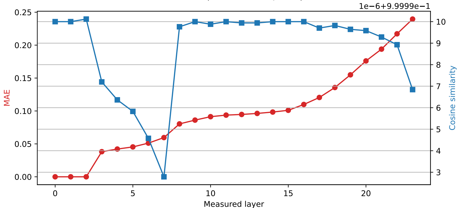
SmolLM2-1.7B-Instruct | Quantized layer 2 | float32 → int8
