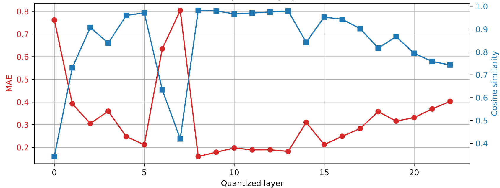
SmolLM2-1.7B-Instruct | Prompt 0 Final RMSNorm output damage | float32 \rightarrow int4
