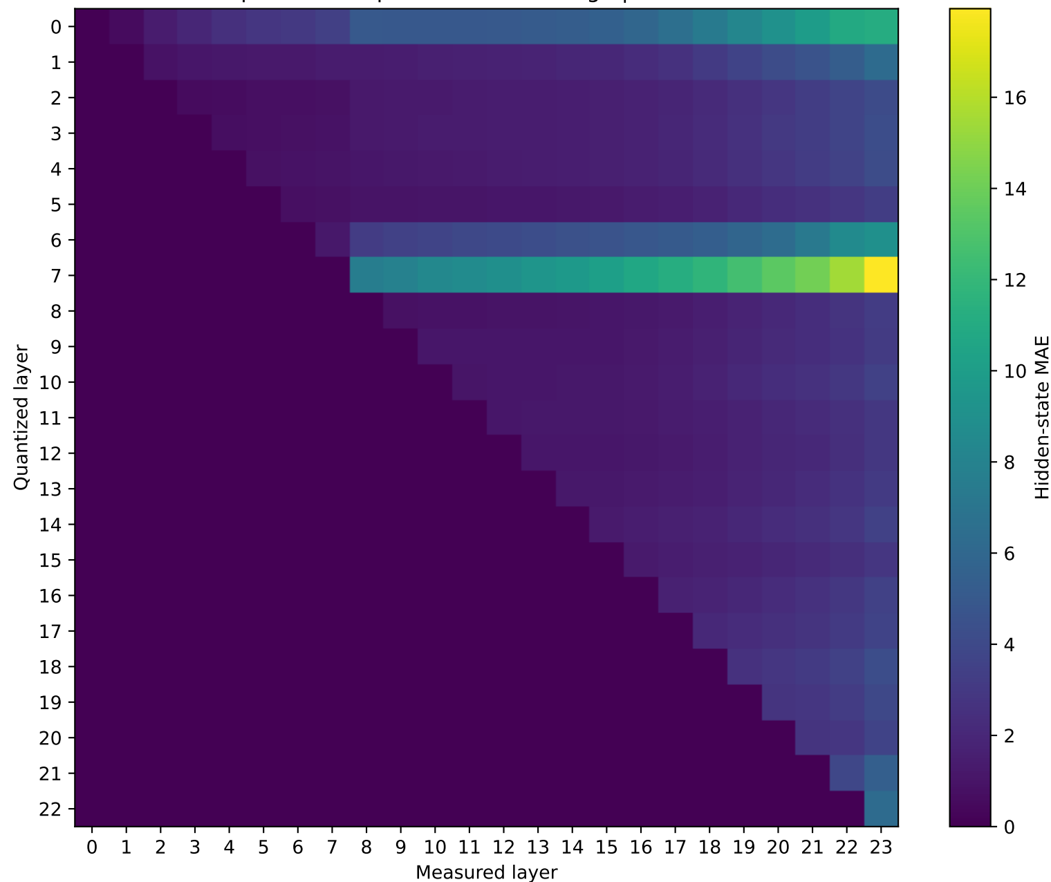
SmolLM2-1.7B-Instruct Prompt 0: MAE representation damage | float32 → int4
