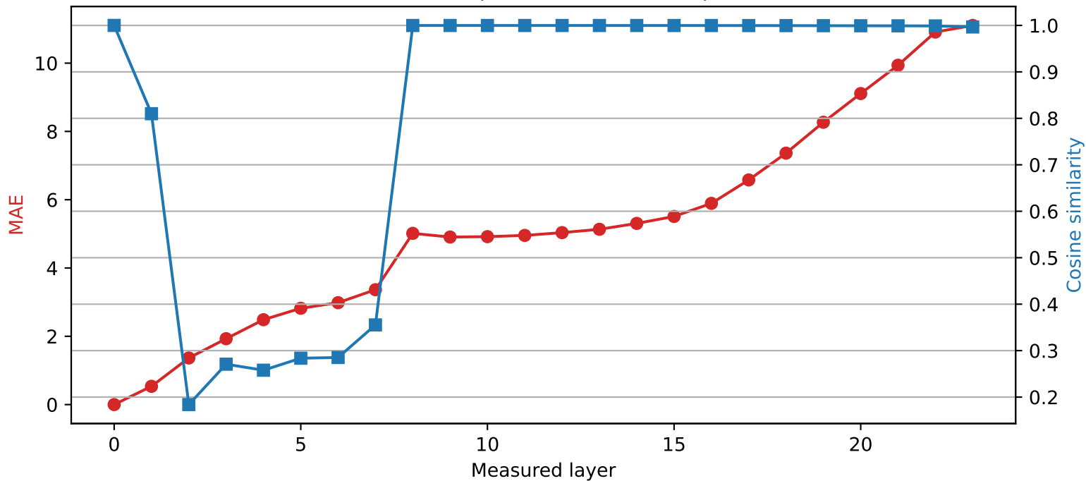
SmolLM2-1.7B-Instruct | Quantized layer 0 | float32 \rightarrow int4
