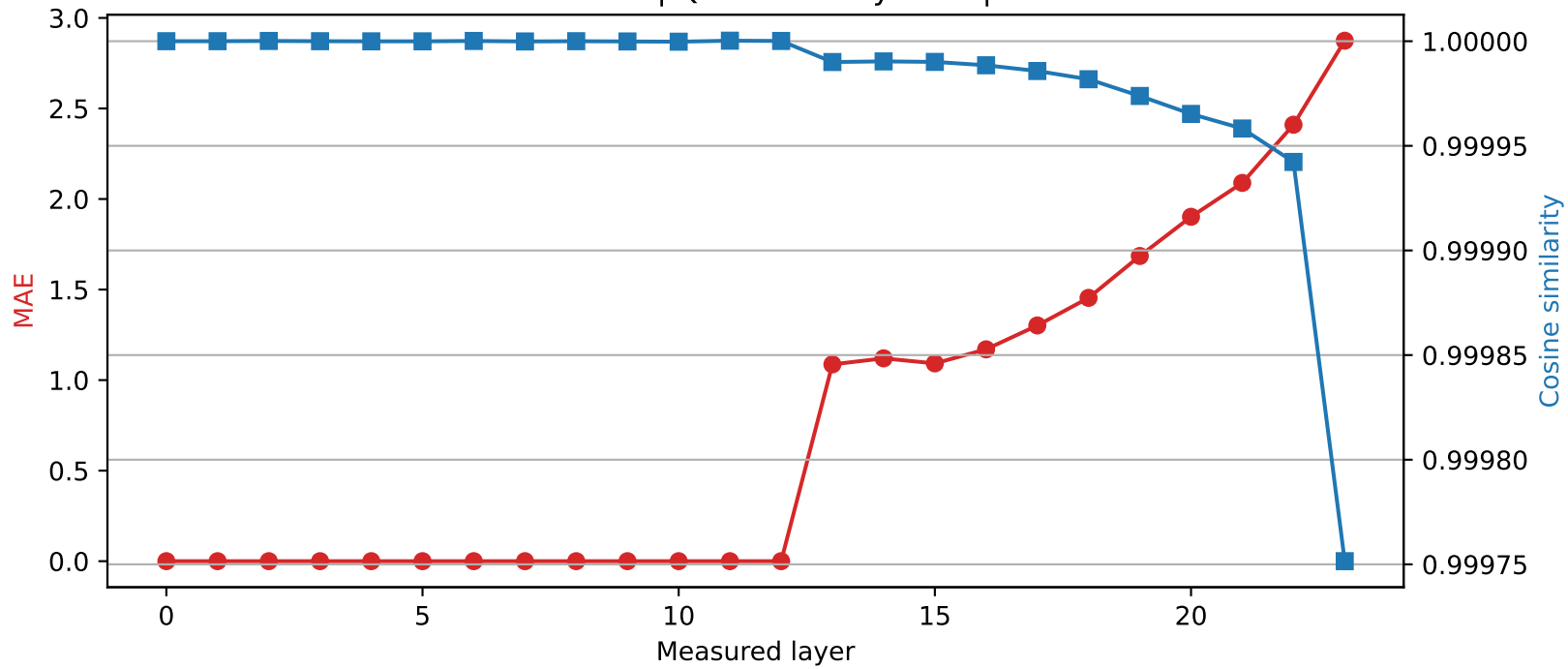
SmolLM2-1.7B-Instruct | Quantized layer 12 | float32 → int4
