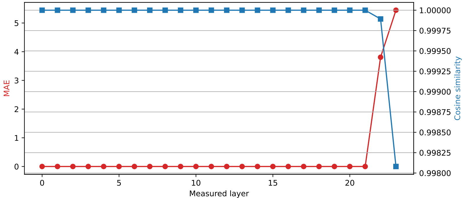
SmolLM2-1.7B-Instruct | Quantized layer 21 | float32 \rightarrow int4
