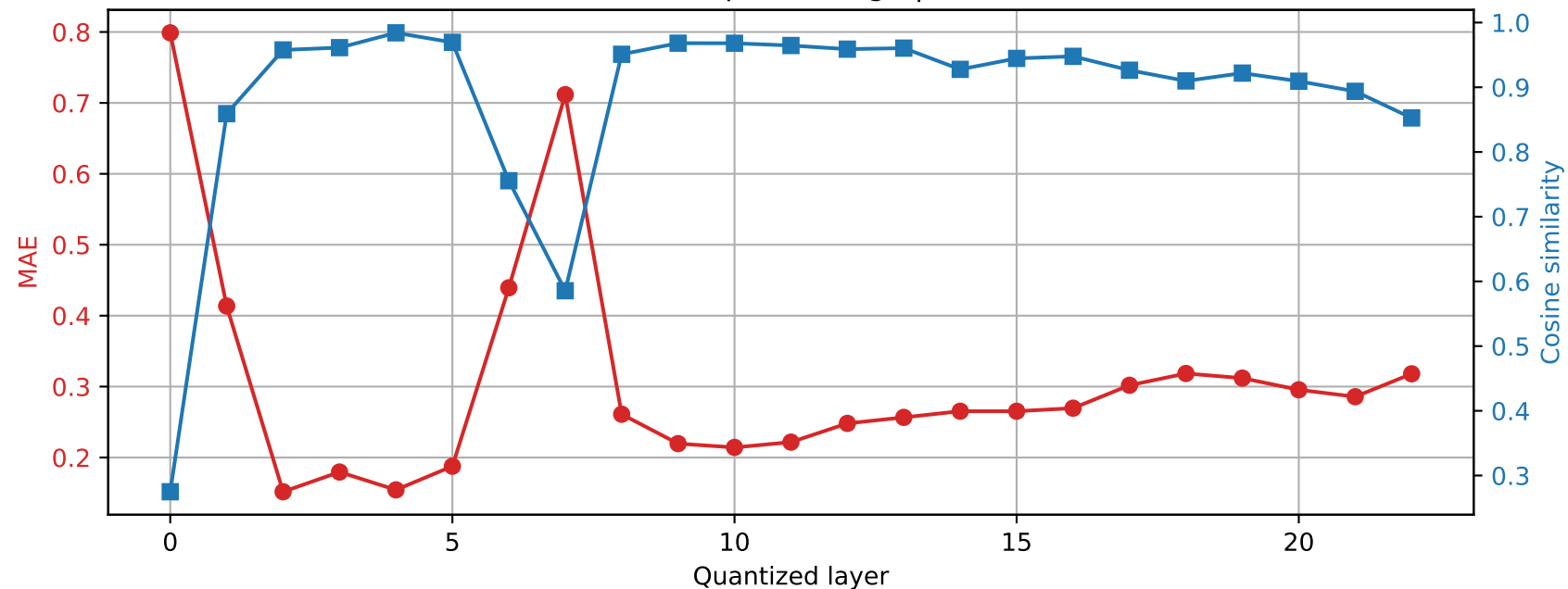
SmolLM2-1.7B-Instruct | Prompt 1 Final RMSNorm output damage | float32 \rightarrow int4
