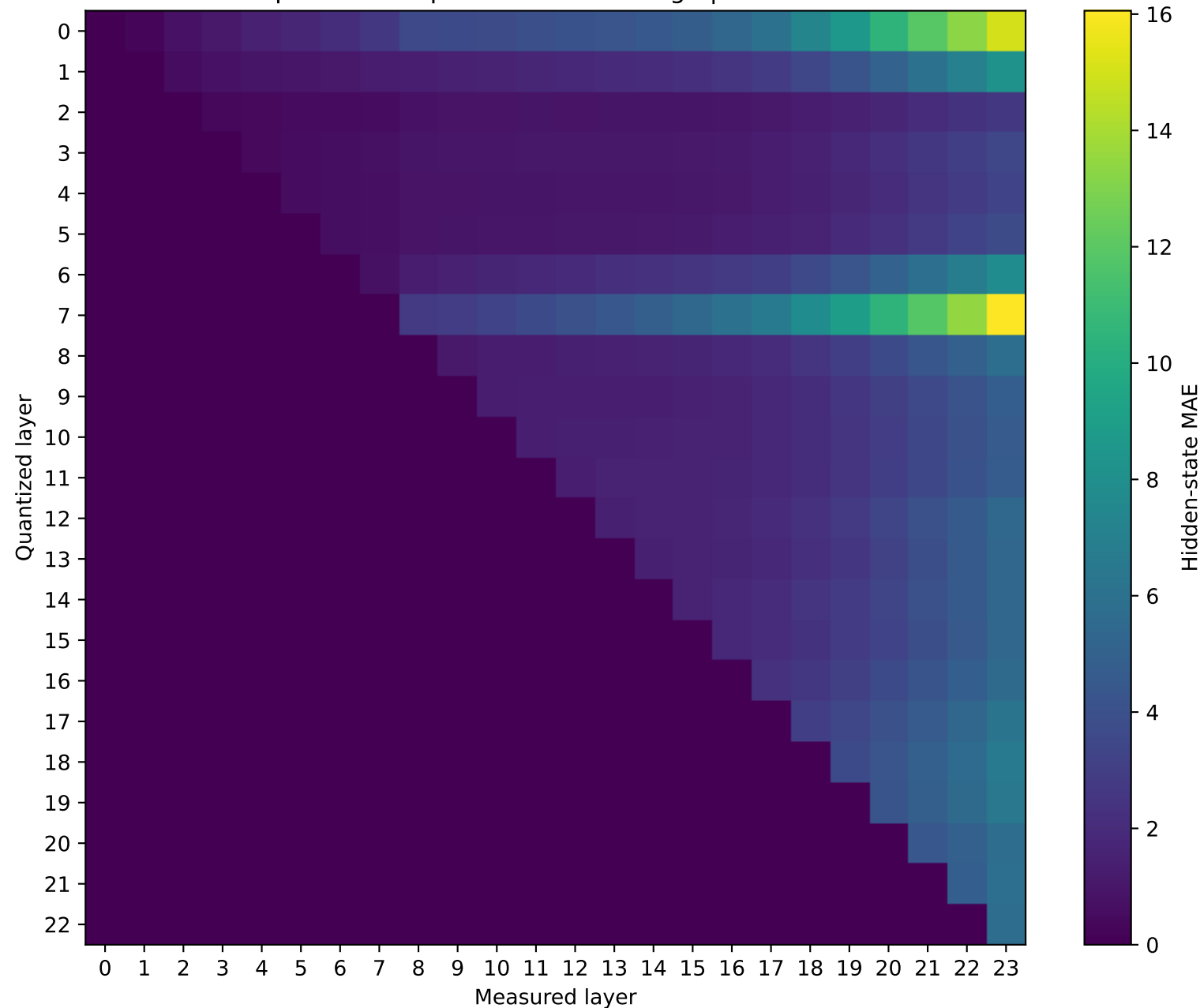
SmolLM2-1.7B-Instruct Prompt 1: MAE representation damage | float32 → int4
