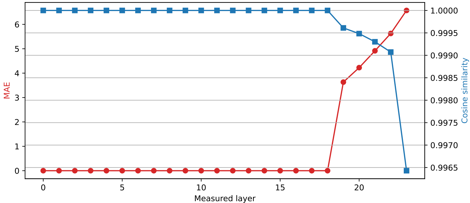
SmolLM2-1.7B-Instruct | Quantized layer 18 | float32 \rightarrow int4
