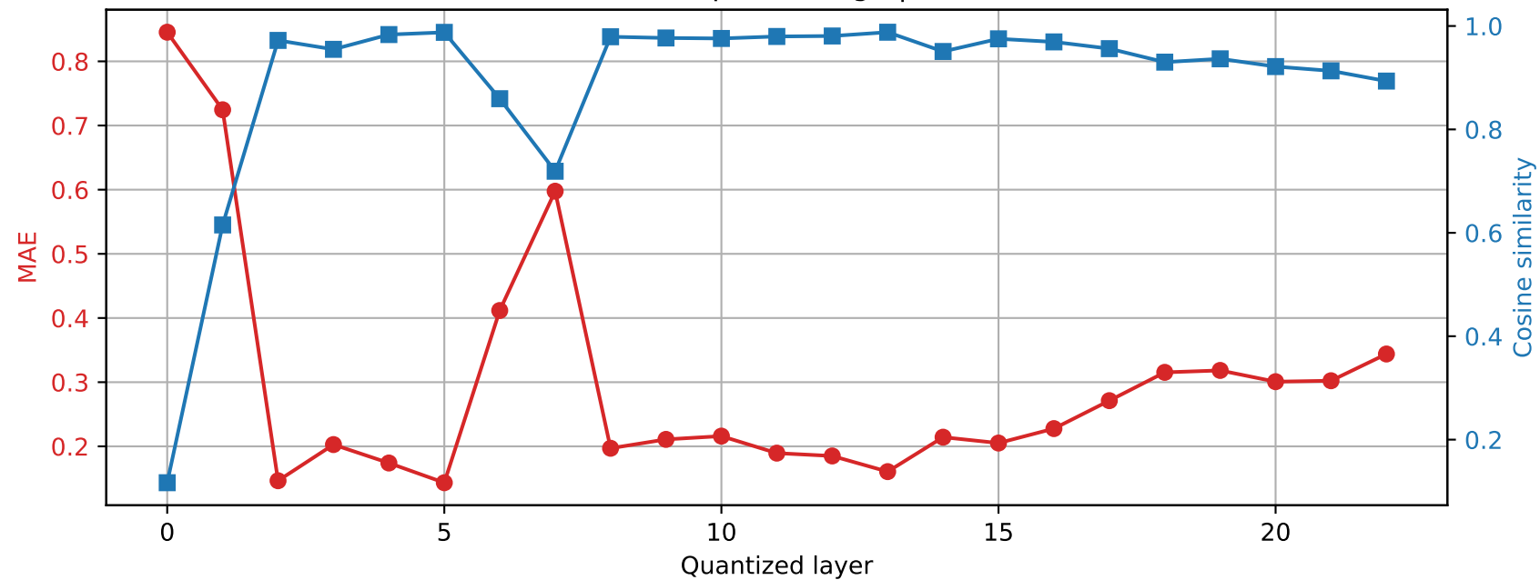
SmolLM2-1.7B-Instruct | Prompt 2 Final RMSNorm output damage | float32 \rightarrow int4
