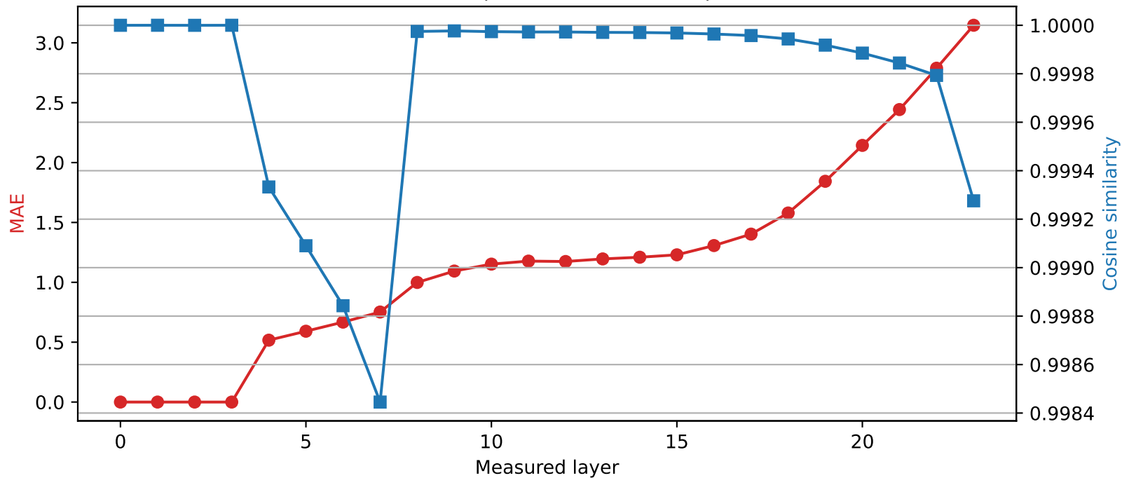
SmolLM2-1.7B-Instruct | Quantized layer 3 | float32 → int4
