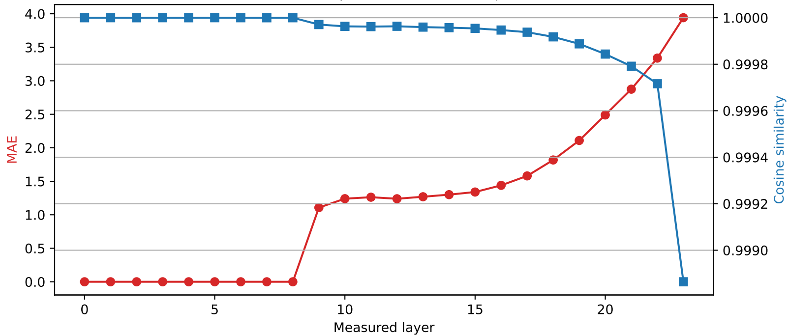
SmolLM2-1.7B-Instruct | Quantized layer 8 | float32 \rightarrow int4
