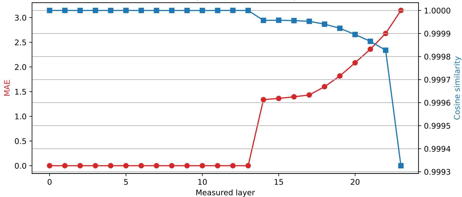
SmolLM2-1.7B-Instruct | Quantized layer 13 | float32 \rightarrow int4
