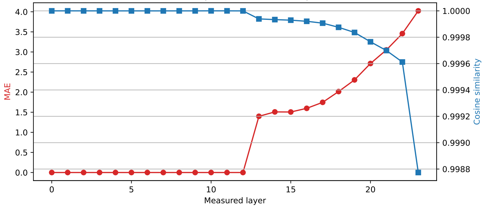
SmolLM2-1.7B-Instruct | Quantized layer 12 | float32 \rightarrow int4
