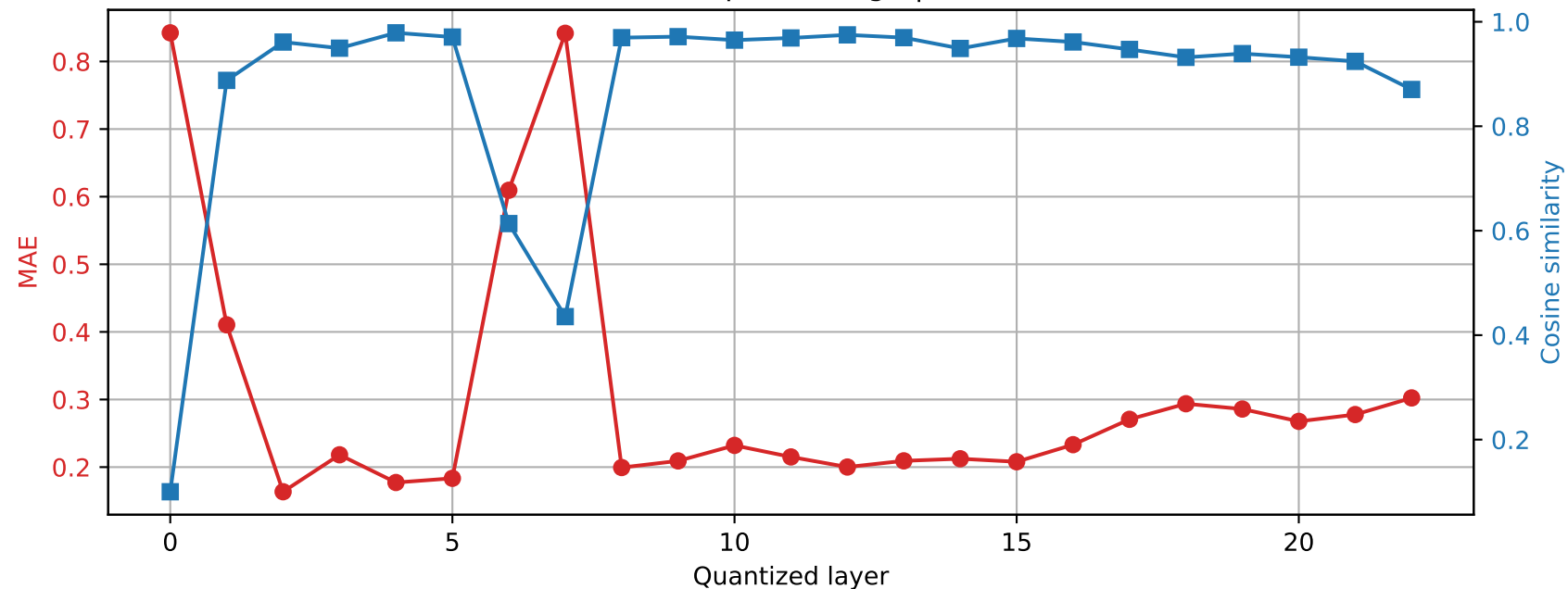
SmolLM2-1.7B-Instruct | Prompt 4 Final RMSNorm output damage | float32 \rightarrow int4
