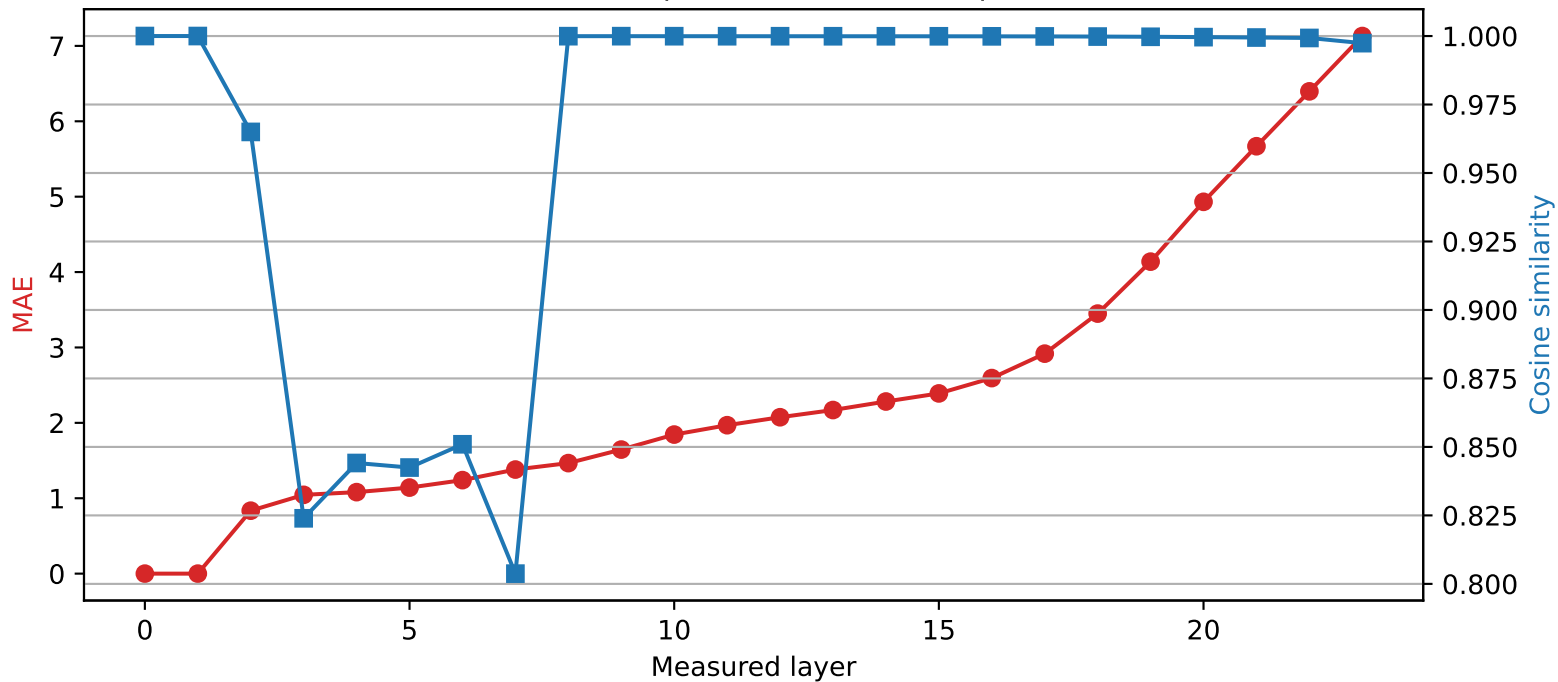
SmolLM2-1.7B-Instruct | Quantized layer 1 | float32 → int4
