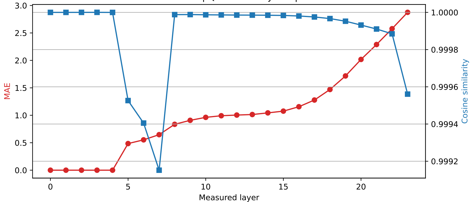
SmolLM2-1.7B-Instruct | Quantized layer 4 | float32 → int4
