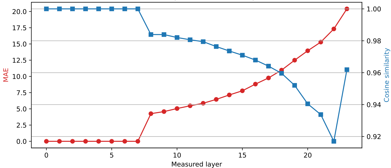
SmolLM2-1.7B-Instruct | Quantized layer 7 | float32 \rightarrow int4
