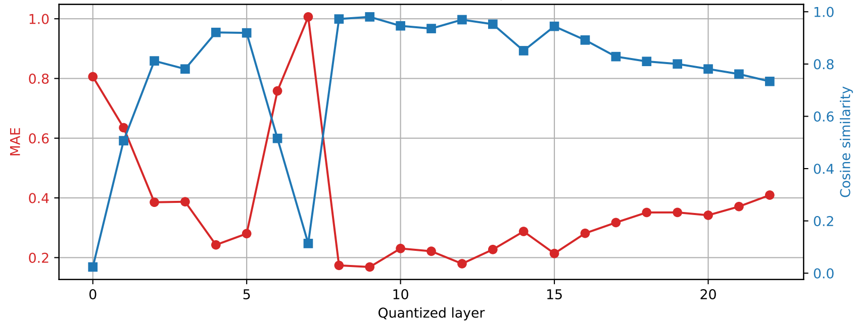
SmolLM2-1.7B-Instruct | Prompt 0 Final RMSNorm output damage | float32 \rightarrow int2
