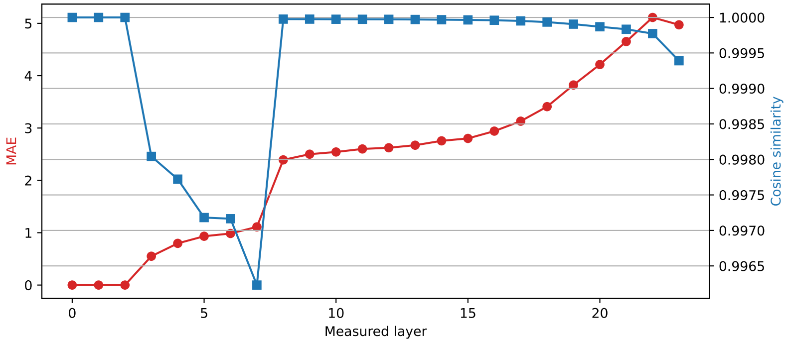
SmolLM2-1.7B-Instruct | Quantized layer 2 | float32 → int2
