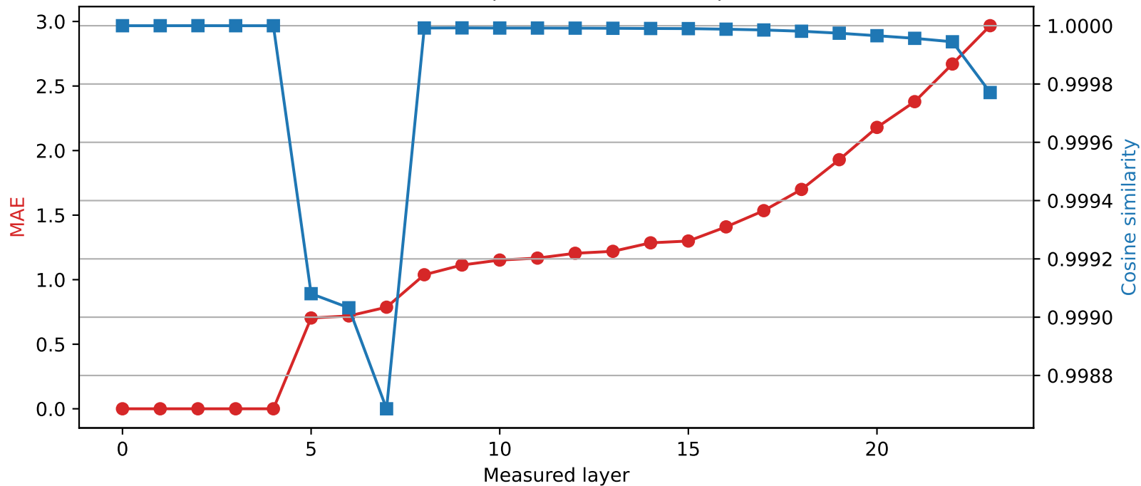
SmolLM2-1.7B-Instruct | Quantized layer 4 | float32 → int2
