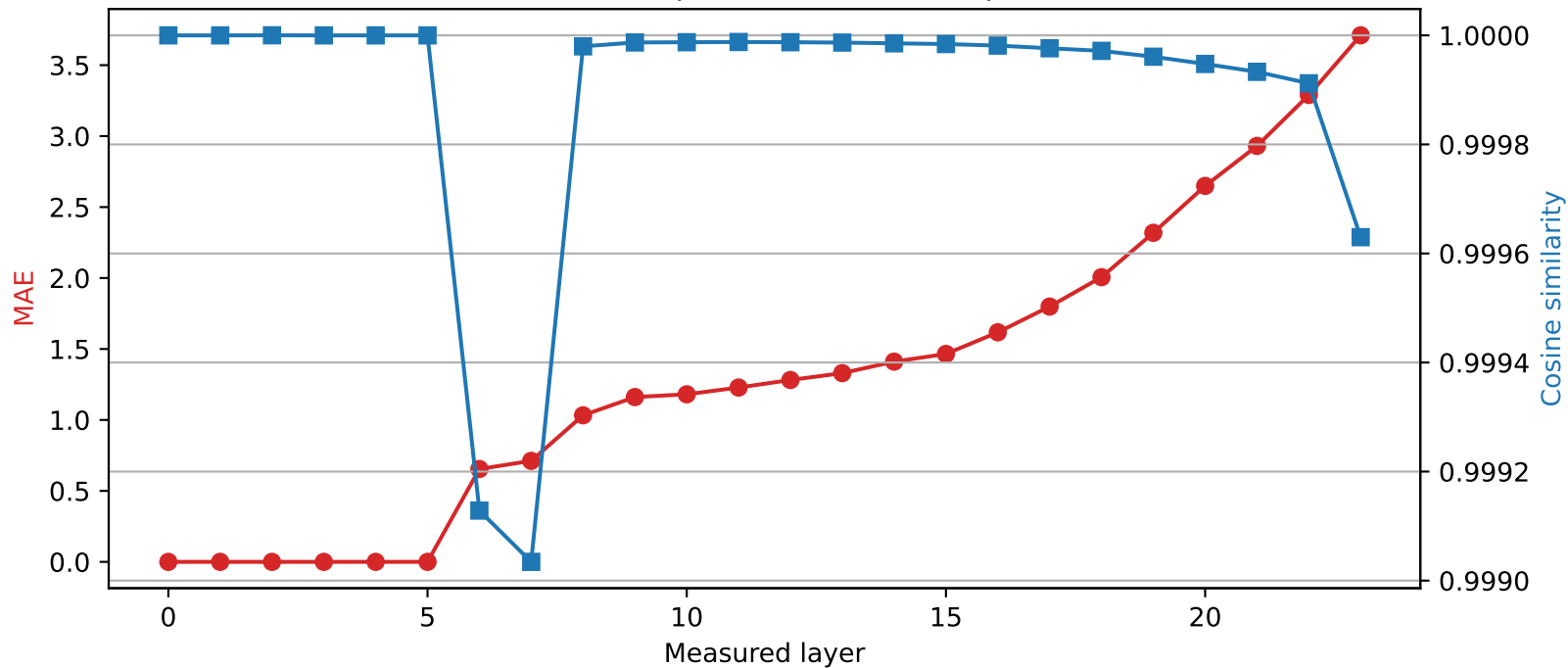
SmolLM2-1.7B-Instruct | Quantized layer 5 | float32 → int2
